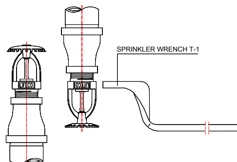
FIGURE D: SPRINKLER WRENCH
