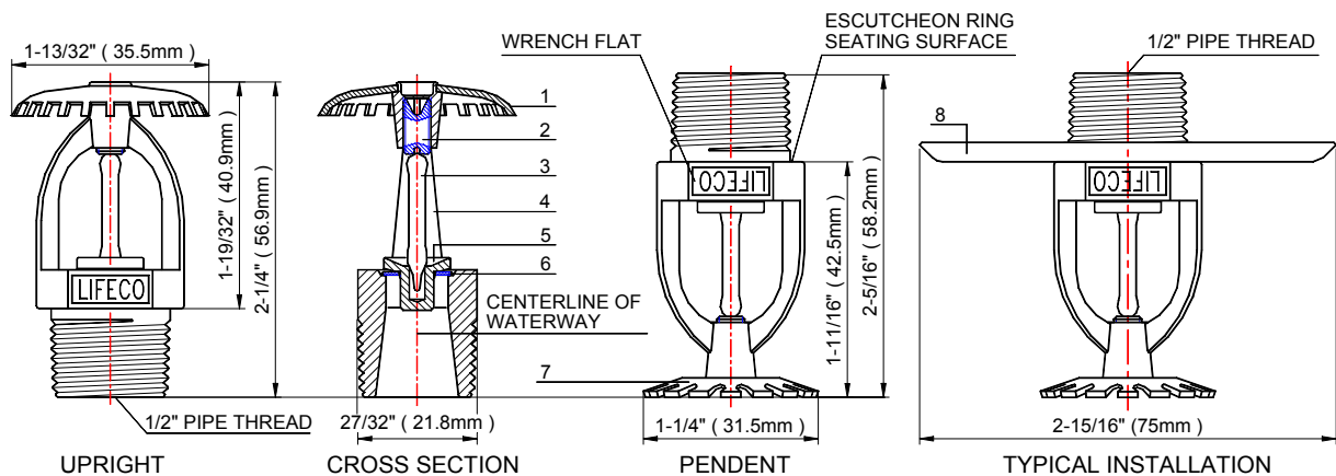
1.SSU DEFLECTOR 2.SET SCREW 3.GLASS BULB 4.FRAME 5.BUTTON 6.SPRING SEAL 7.SSP DEFLECTOR 8.STANDARD ESCUTCHEON
