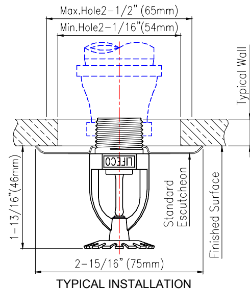
FIGURE C: MODEL LIFECO005/LIFECO006 PENDENT SPRINKLER INSTALLED WITH A STANDARD ESCUTCHEON
