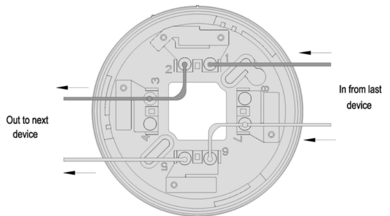
Figure 2: Loop Powered
