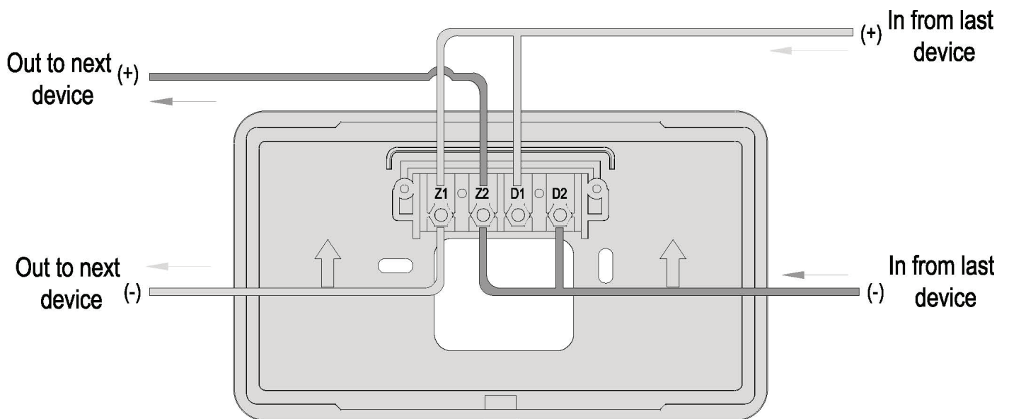
Loop Powered Wiring Details
