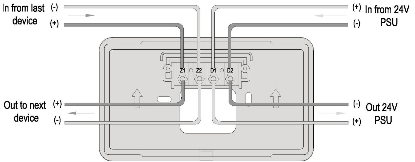
With External Supply Wiring Details
