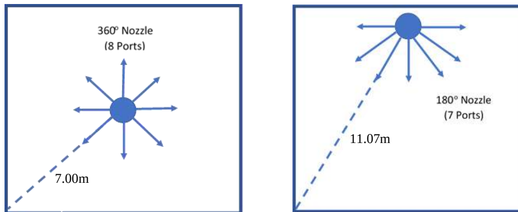
Figure 33 180° & 360° Nozzle Radius
