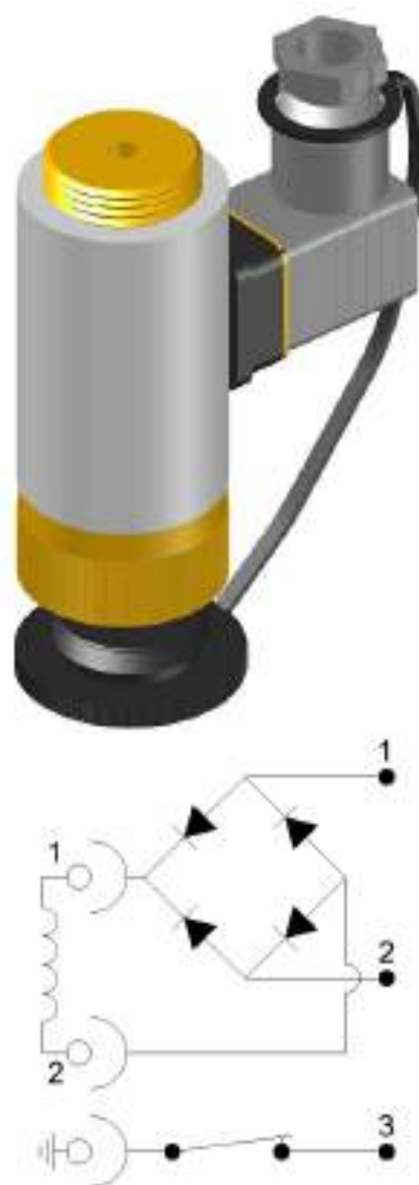
Figure 5 Electrical Actuator Complete with Supervision Switch & Wiring Diagram
