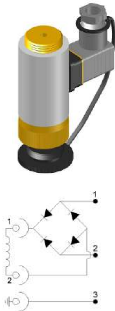
Figure 16 Electrical Actuator & Wiring Diagram
