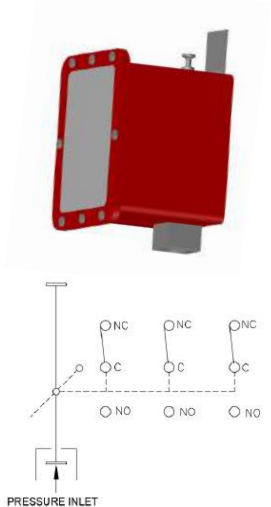
Figure 22 Discharge Pressure Switch & Wiring Diagram
