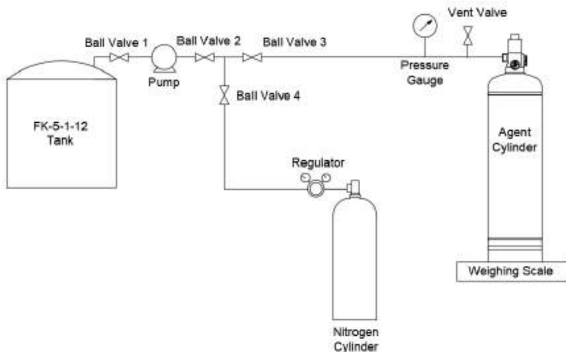
Figure 58: Filling Station Example Set Up
