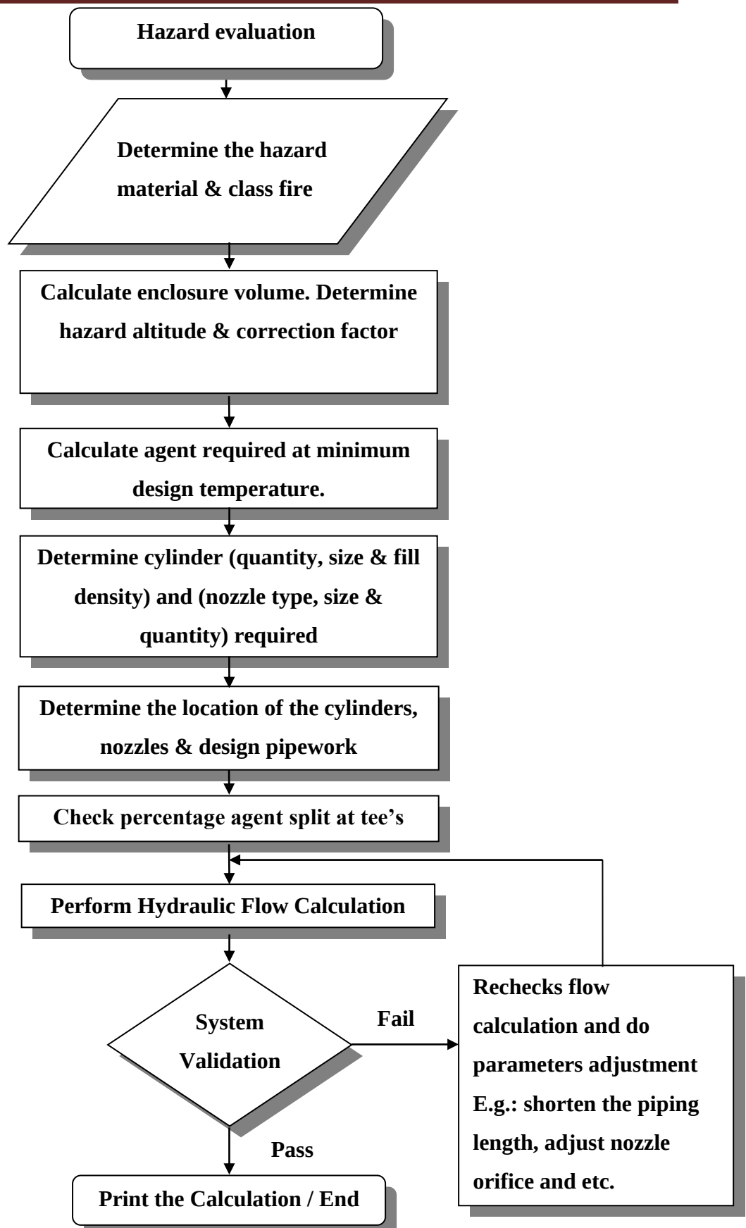
Figure 39 System Design Flow Chart
