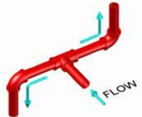
Figure 28 Correct Bull Tee Splits Orientation
