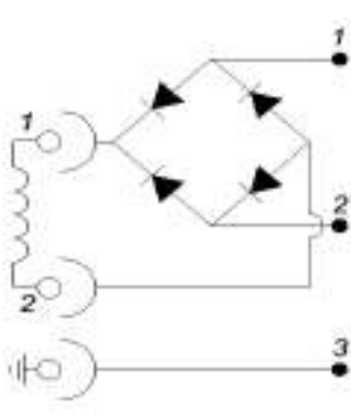
Electrical Actuator (Bridge Rectifier) LF-EASV
