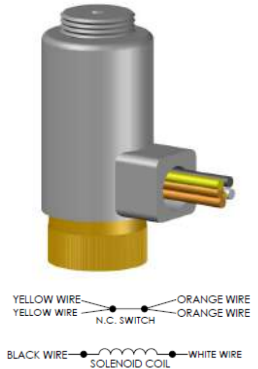
Figure 6 Electrical Actuator Complete with Supervision Switch & Wiring Diagram
