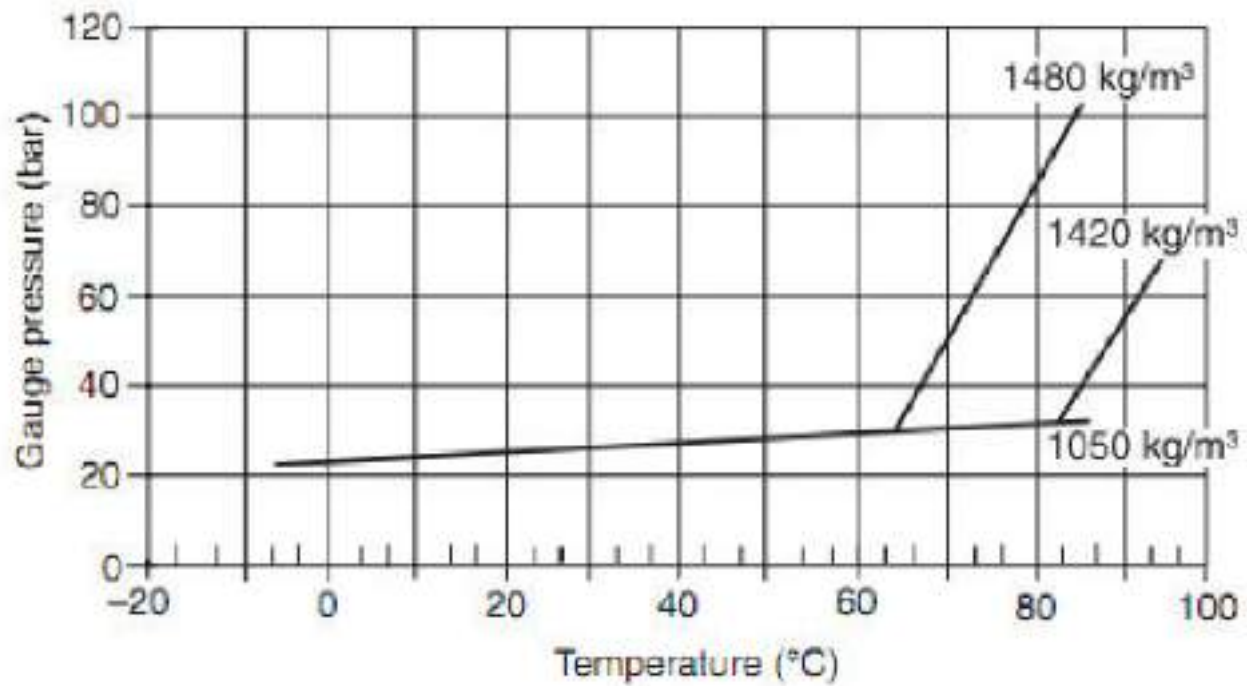
ISOMETRIC DIAGRAM OF FK5-1-12 PRESSURIZED TO 25 BAR, GAUGE AT 20 °C
