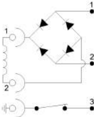
Removable Electrical Actuator c/w Supervision switch LF-EASV-RS
