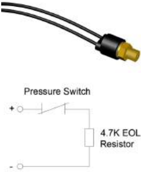
Figure 23.2 Low Pressure Switch & Wiring Diagram
