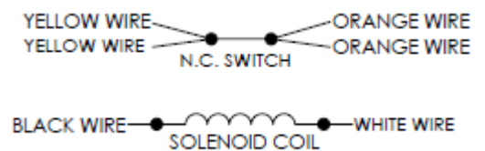
Figure 6 Electrical Actuator Complete with Supervision Switch & Wiring Diagram
