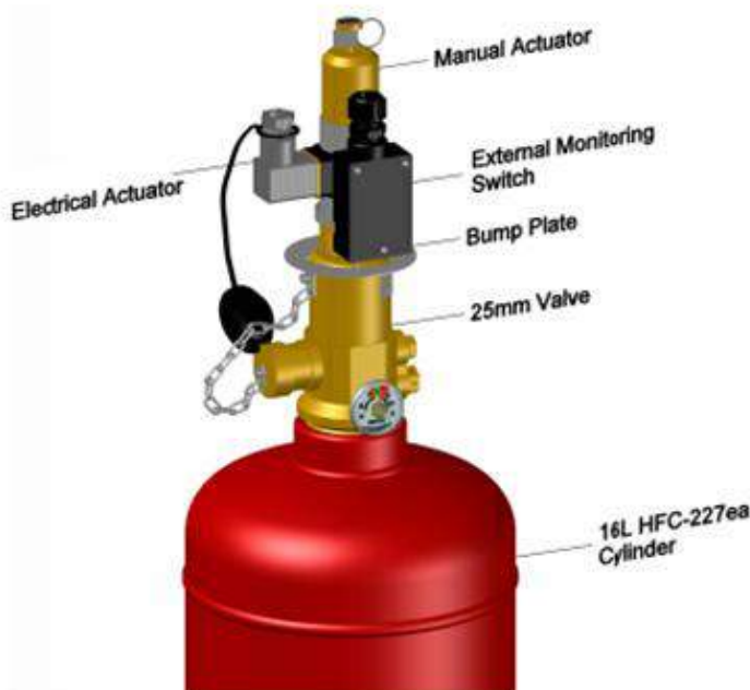
Figure 49 (a): Installation of External Monitoring for 1 inch & 2 inch Cylinder Valve.
