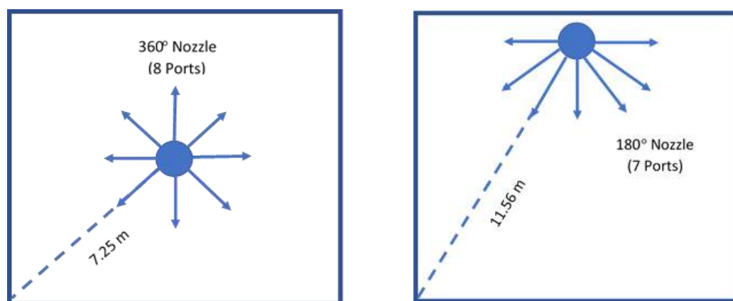
Figure 33 180° & 360° Nozzle Radius
