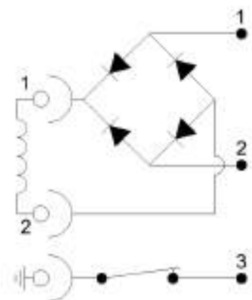
Figure 5 Electrical Actuator Complete with Supervision Switch & Wiring Diagram
