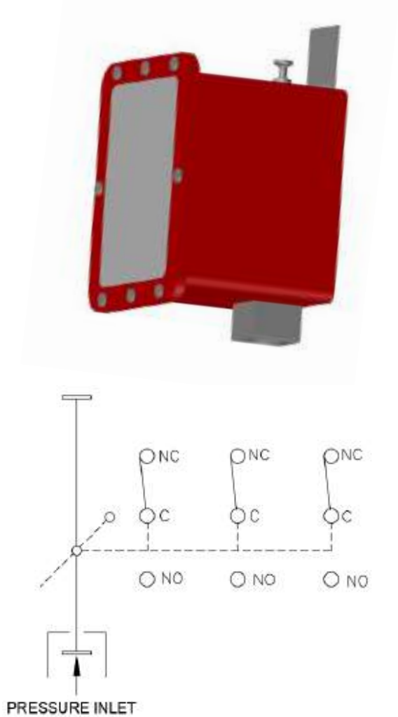
Figure 23.1 Discharge Pressure Switch & Wiring Diagram
