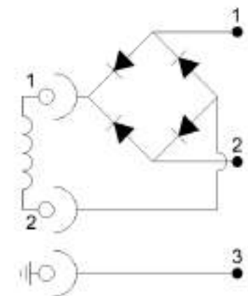
Figure 16 Electrical Actuator & Wiring Diagram
