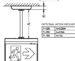
HANGING INSTALLATION (unit: mm)
